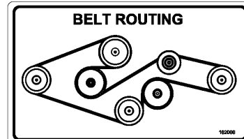
Part No. 162066
