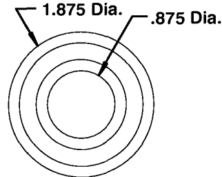
PART NO. 120070
